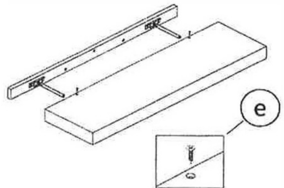
Step 5: Attach floating shelf with shelf brackets. Install with screws (e 3.5*19=3 pcs)
