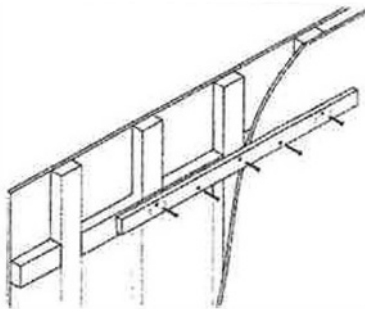
Step 1: Locate install space. Install supporting rod to wall studs
