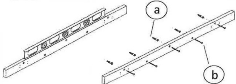
Step 2: Adjust level then install wood supporting rod with long screws.
