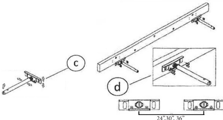
Step 3: Adjust shelf brackets (5 way adjustable)
