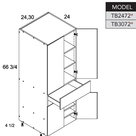
Tall Four Door One Drawer Utility
